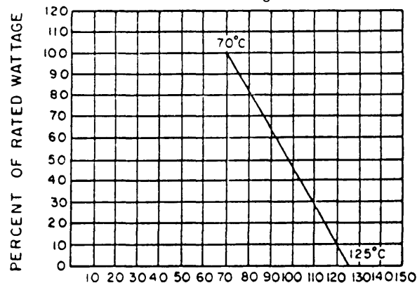
FIGURE 209-1. Derating curves for high ambient temperatures.
