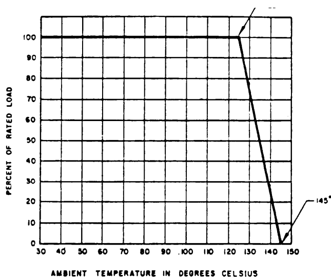
FIGURE 303-1. Derating curve for high ambient temperature.
