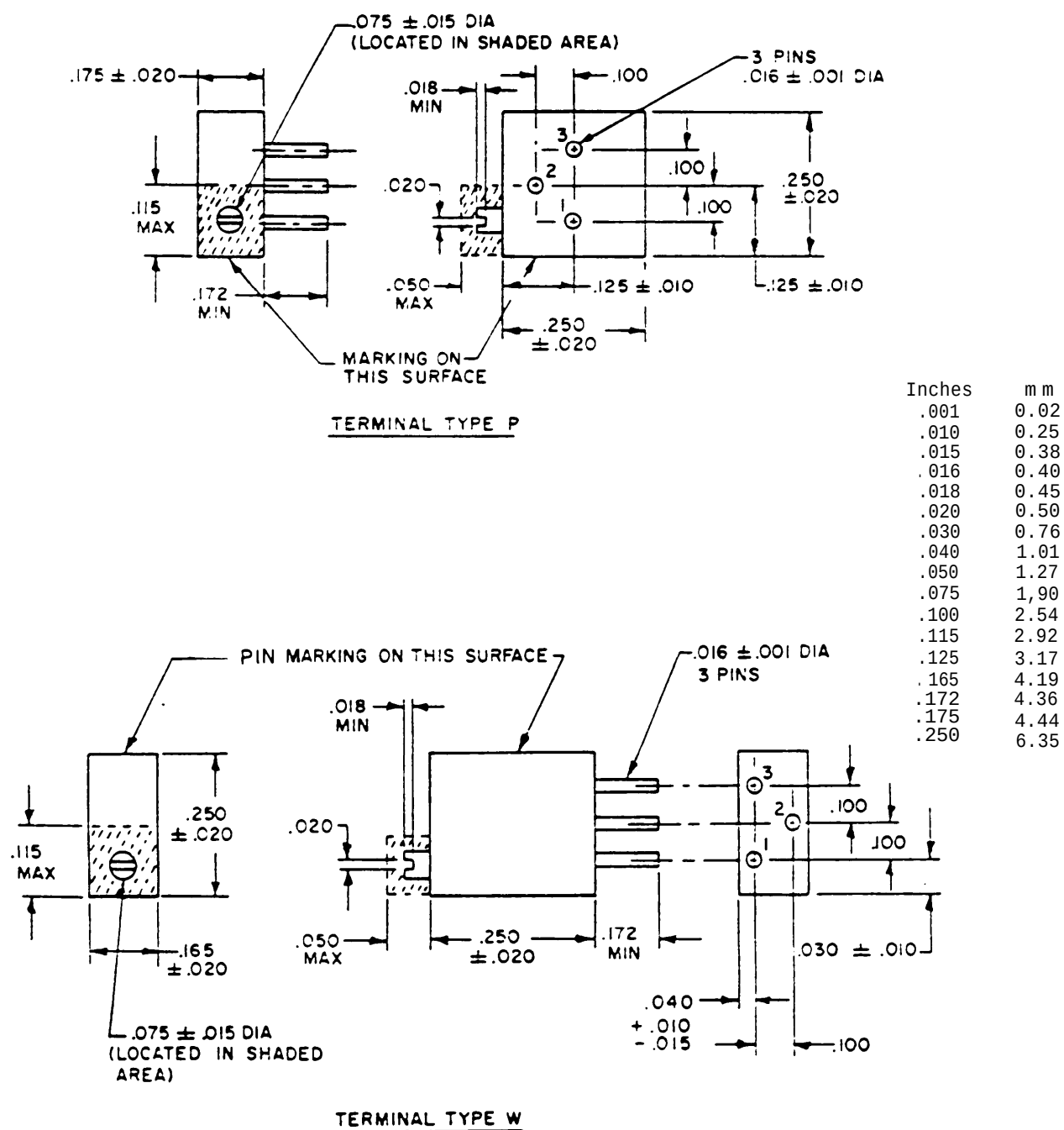
FIGURE 402-3. Established reliability, adjustment type, nonwirewound, variable resistors - Continued.
