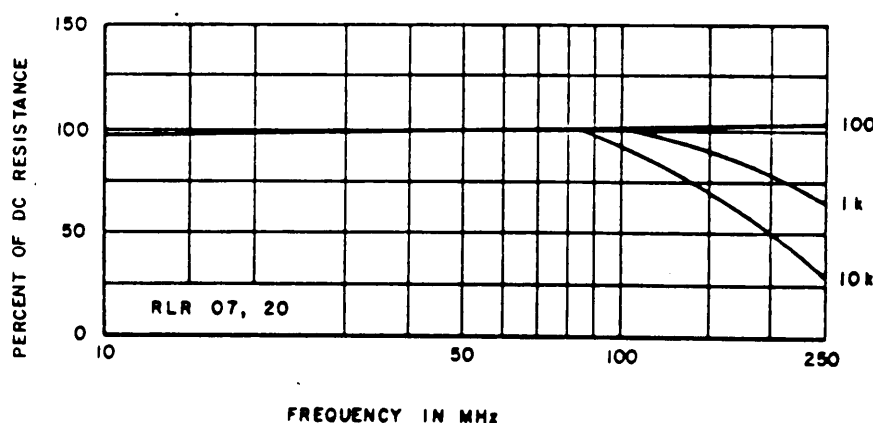
FIGURE 305-2. Response curve.
