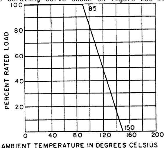
FIGURE 206-1. Derating curve for high-ambient temperature.
