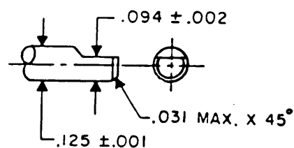
FLATTED SHAFT
