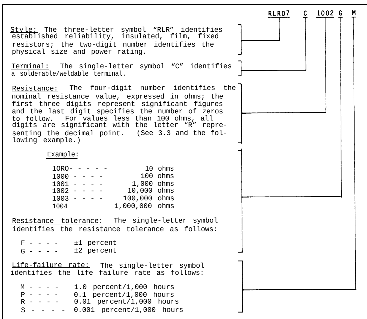
FIGURE 305-3. Type designation example.
