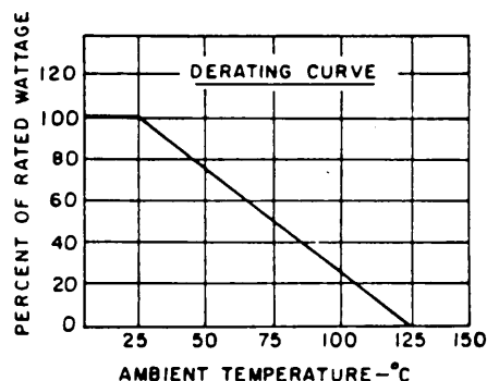
FIGURE 502-I. Power ratings and derating curve.
